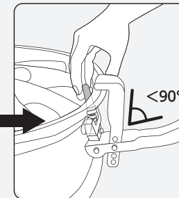
Hold rubber valve stem and make sure angle is less than 90 degree
